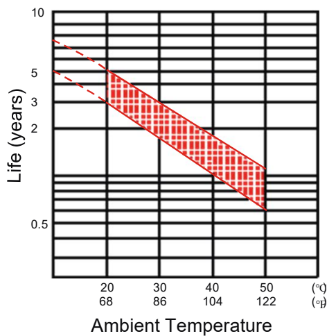
Trickle (or float) Service Life
