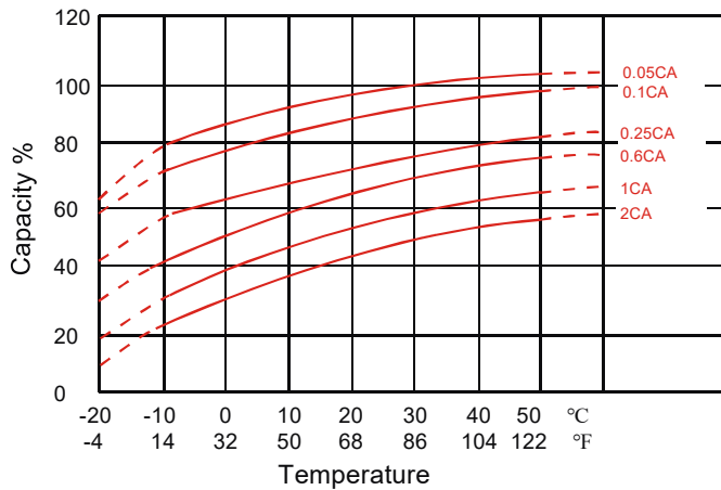
Effect of Temperature on Capacity 25°C °F (77 °F)
